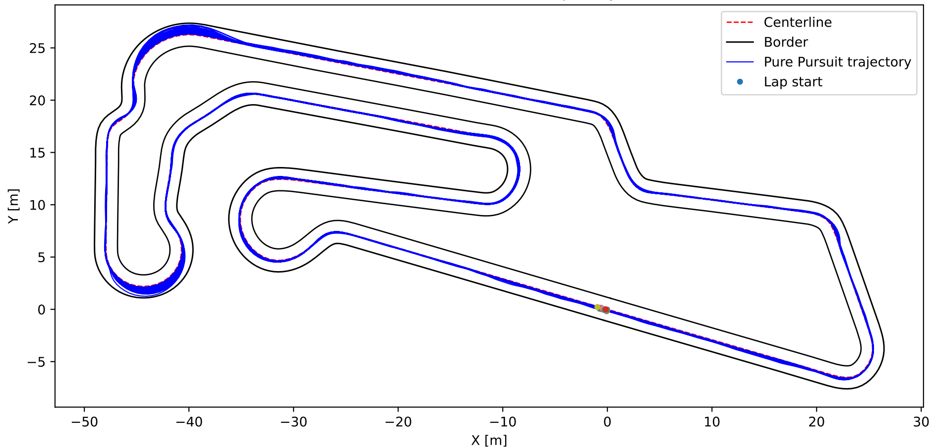
Pure Pursuit Collected Trajectory
