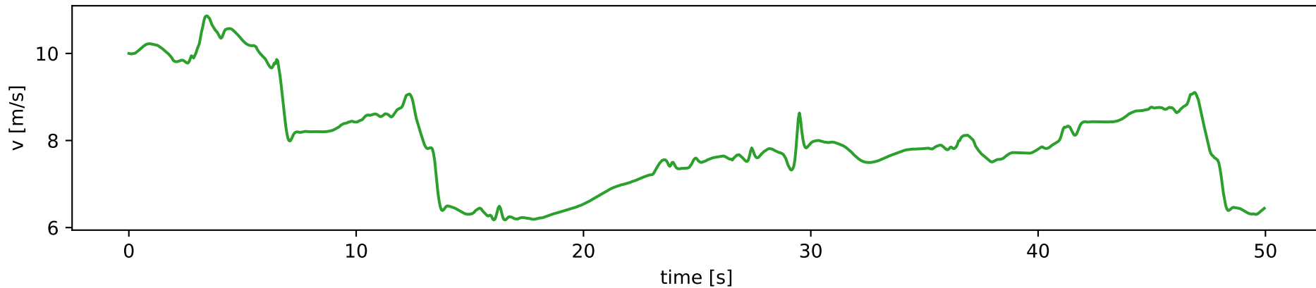
Velocity — C-MIMO DeepONet (proposed)+PANOC MPCC
