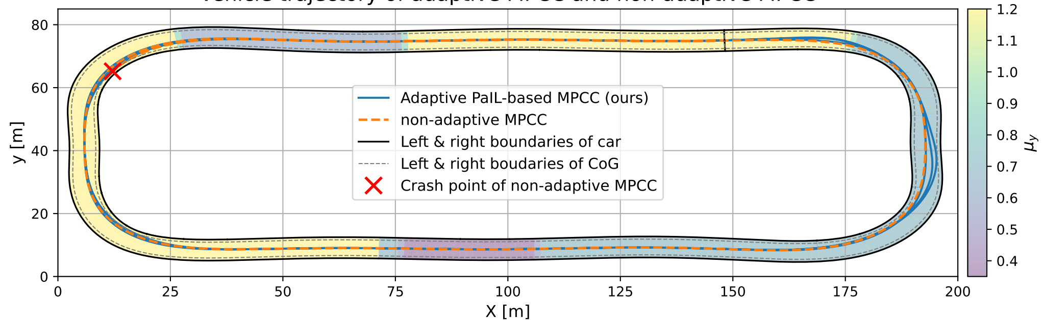
Vehicle trajectory of adaptive MPCC and non-adaptive MPCC
