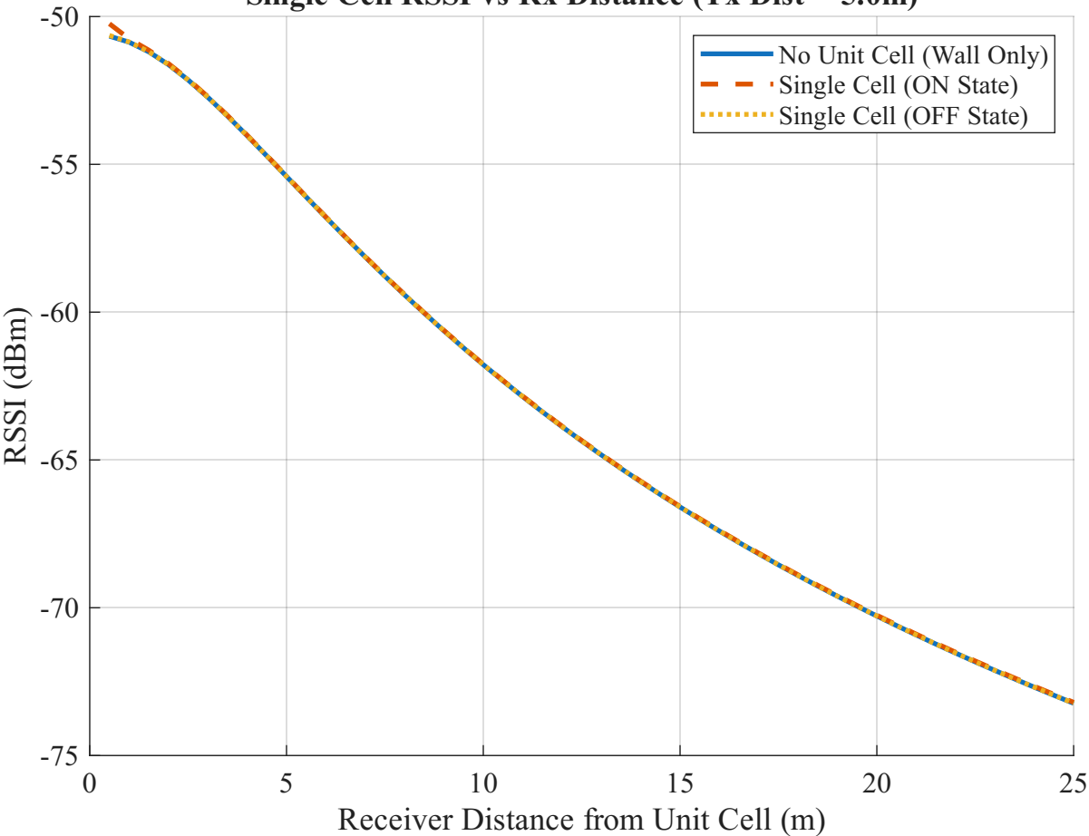
Single Cell RSSI vs Rx Distance (Tx Dist = 5.0m)
