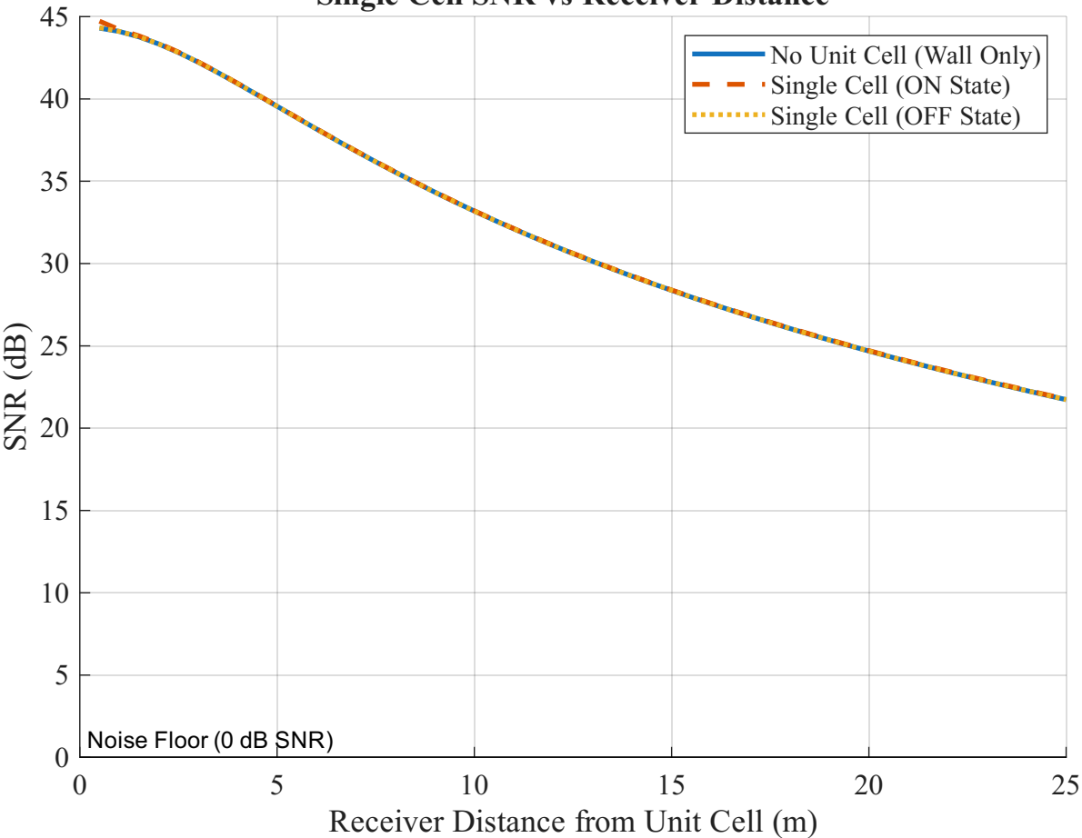
Single Cell SNR vs Receiver Distance
