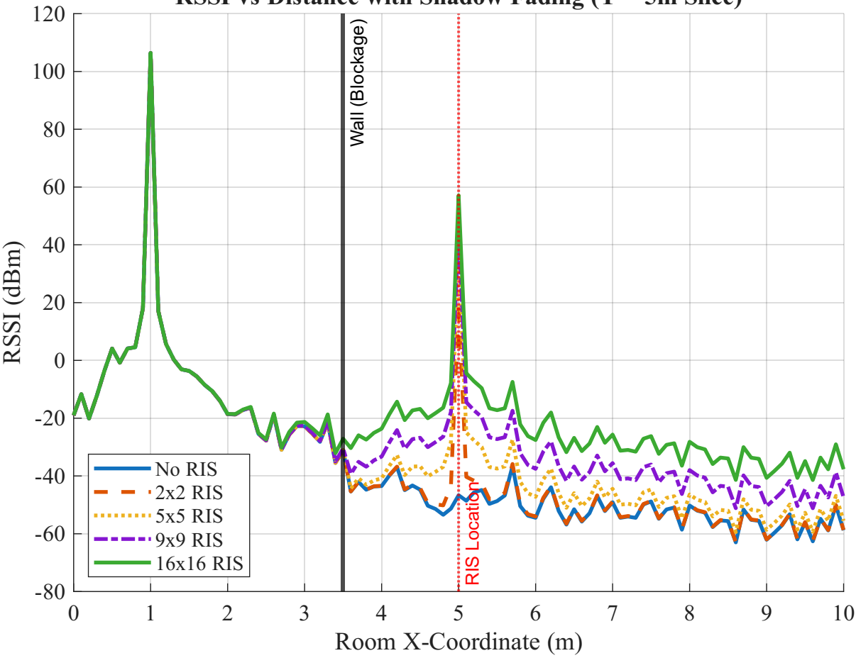
RSSI vs Distance with Shadow Fading (Y = 5m Slice)
