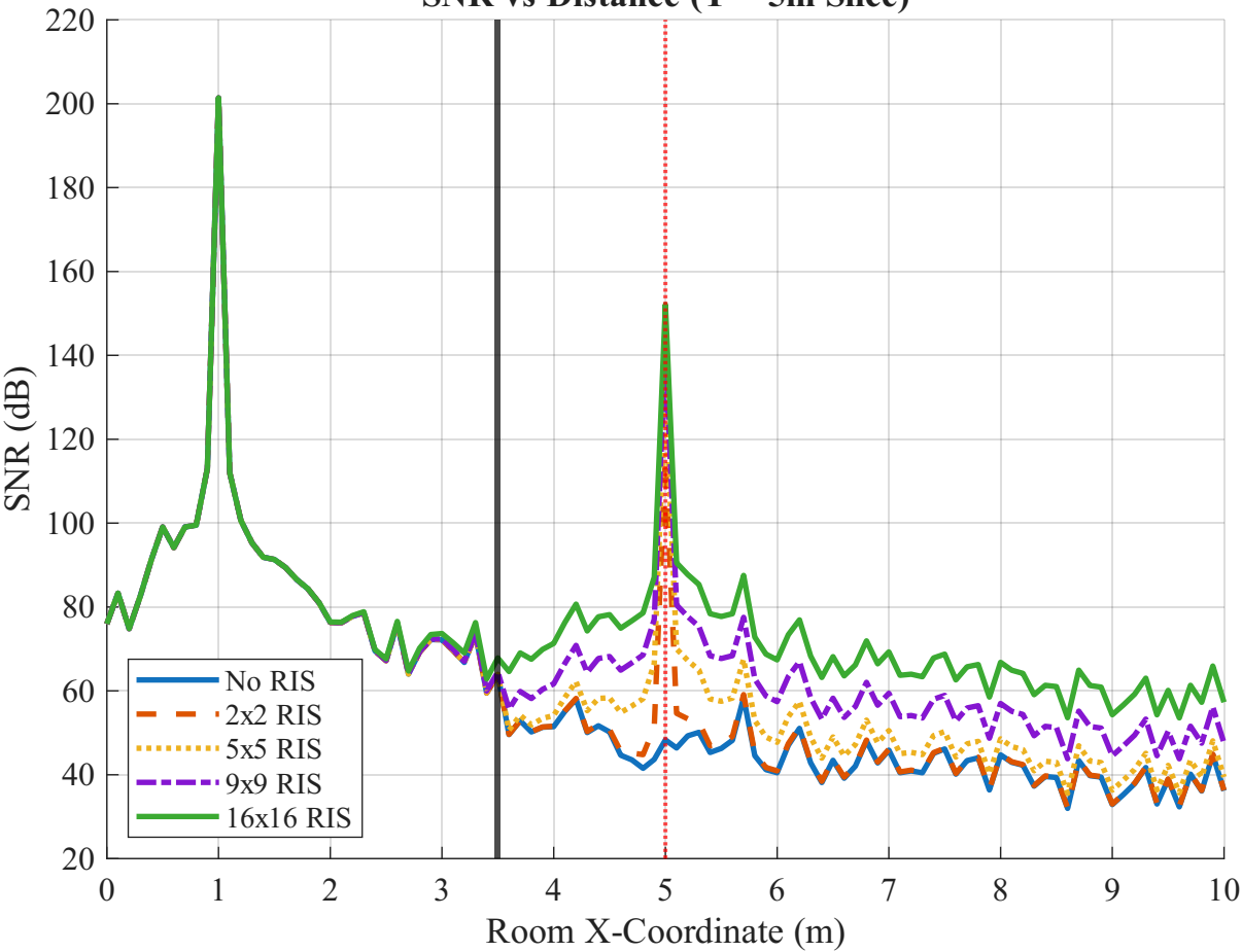
SNR vs Distance (Y = 5m Slice)
