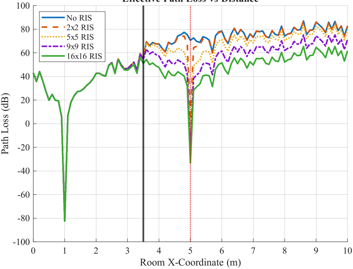
Effective Path Loss vs Distance
