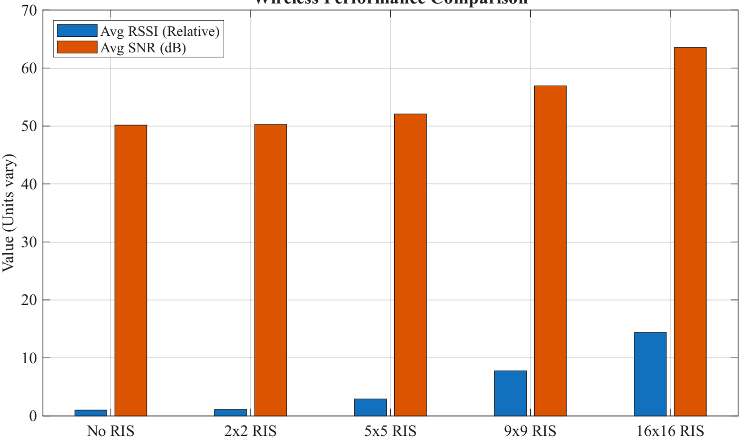
Wireless Performance Comparison
