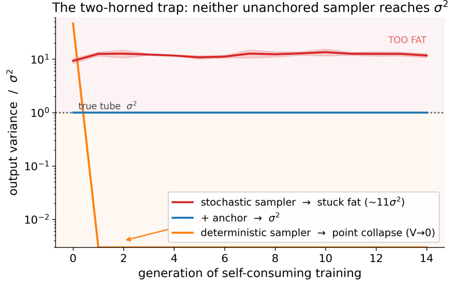
Figure 2: The two-horned trap ( we observe ) . Self-consuming recursions at fixed t_0 = 10^{-4} , no anchor, 3 seeds. With the reverse-SDE noise on, the recursion sticks fat at 10.8\text{--}13.2\sigma^2 (red). With the noise zeroed (deterministic sampler), it collapses to a single point within one generation (orange; verified loss of all 2-D spread, no numerical overflow). Neither branch reaches the tube ( \sigma^2 , dotted); the anchored recursion (blue, Section 6) holds it.
