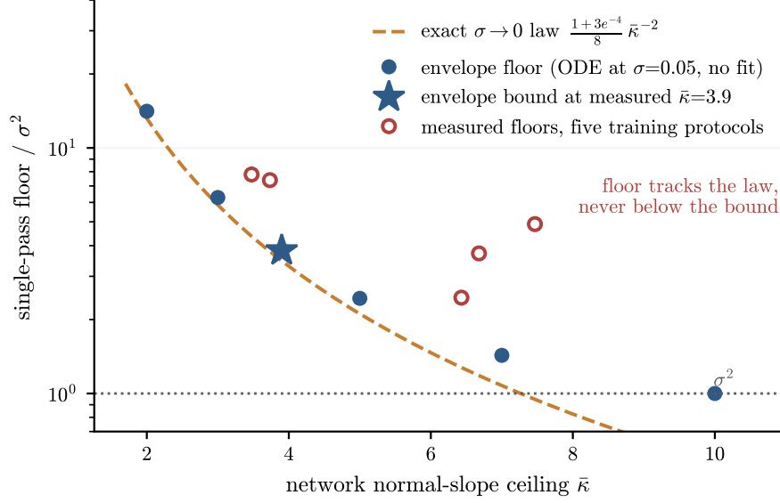
Figure 3: The capacity floor: predicted, measured, and moved. Filled blue: finite- \sigma variance-ODE envelope floor at \sigma = 0.05 (no fit). Dashed: the exact \sigma \rightarrow 0 law \frac{(1 + 3e^{-4})}{8} \bar{\kappa}^{-2} of Theorem 2. Star: the envelope bound 3.8\sigma^2 at the standard pipeline’s measured ceiling \bar{\kappa} = 3.9 — a proven lower bound that accounts for \sim 60\% of the directly measured single-pass floor; the measured anatomy of the remainder (profile sag, ensemble displacement) is in the text. Open circles: the interventional test — five training protocols move the measured ceiling from 3.5 to 7.5 and the measured floor falls from 7.8 to 2.5\sigma^2 , tracking the law and never crossing the bound.
