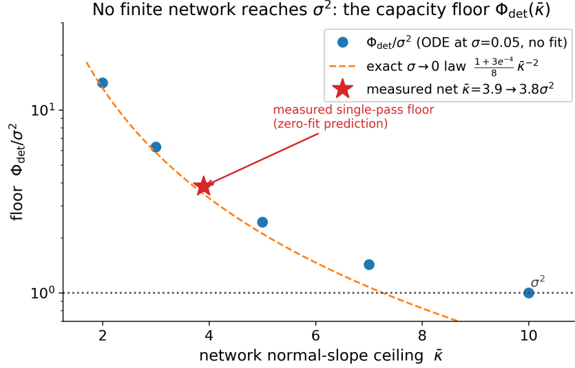
Figure 3: The capacity floor, predicted and measured. Blue: finite- \sigma variance-ODE floor at \sigma = 0.05 (no fit). Dashed: the exact \sigma \rightarrow 0 law ((1 + 3e^{-4})/8)\bar{\kappa}^{-2} of Theorem 2. Star: the envelope floor 3.8\sigma^2 at the measured ceiling \bar{\kappa} = 3.9 — a proven lower bound that accounts for \sim 60\% of the directly measured single-pass floor; the measured anatomy of the remainder (profile sag, ensemble displacement) is in the text.
