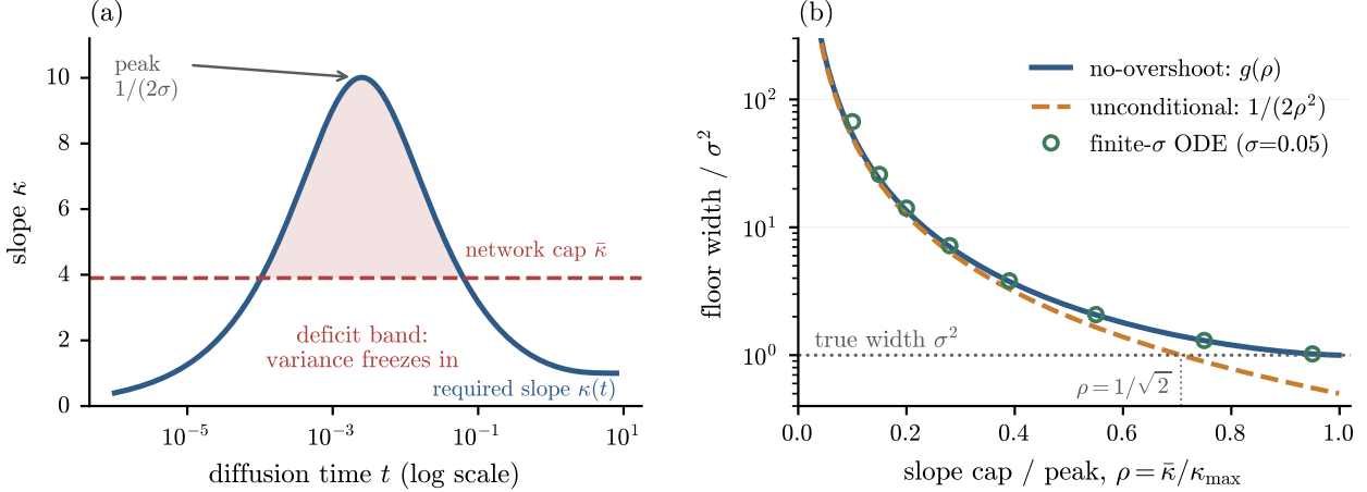
Figure 1: The mechanism and the law. (a) The required normal slope \kappa(t) = s/\gamma^2 is non-monotone: it peaks at \kappa_{\max} = 1/(2\sigma) near t \approx \sigma^2 and falls back to zero. A network with ceiling \bar{\kappa} < \kappa_{\max} under-contracts only on a finite band (shaded, the cap-to-curve deficit lens); variance frozen in the band cannot be removed below it (too few contraction e-folds remain). (b) The resulting floor in units of \sigma^2 as a function of \rho = 2\sigma\bar{\kappa} : closed-form no-overshoot law g(\rho) (blue, Theorem 2), exact unconditional law 1/(2\rho^2) (orange). Green rings: direct finite- \sigma ODE integration at \sigma = 0.05 swept across \rho (self-checked against the appendix triples), sitting just above g(\rho) and following the no-overshoot branch, the relative O(\sigma^2/\rho^2) convergence the theorem predicts. The dotted vertical marks \rho = 1/\sqrt{2} , below which the floor exceeds the true width \sigma^2 .
