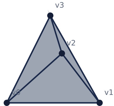
3-simplex tetrahedron
