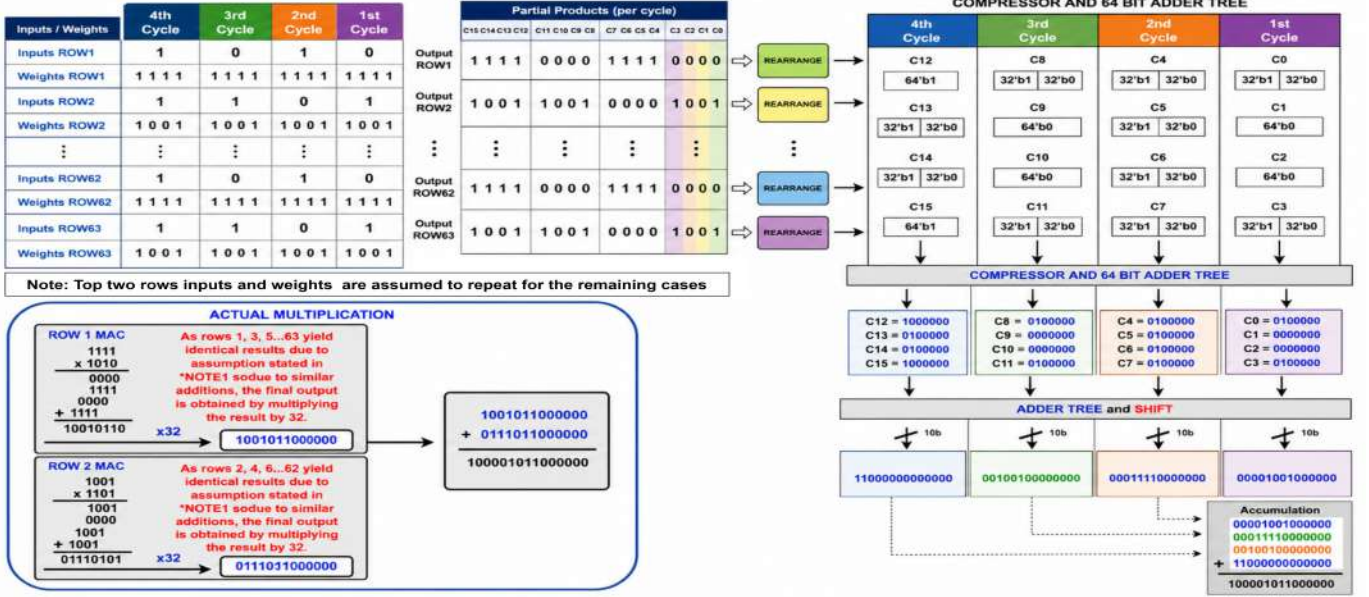
Fig. 11: Dataflow of a 2-D vector dot product using the logical structure of a scaled-down 2-bank macro. The timing waveforms over four cycles illustrate partial-product generation, adder-tree accumulation, and shift-accumulation, producing the final result after five clock cycles.
