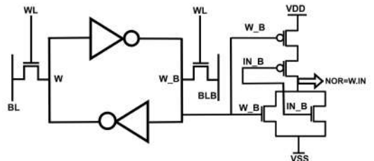
Fig. 2: NOR-enabled SRAM bitcell used in Proposed CIM
