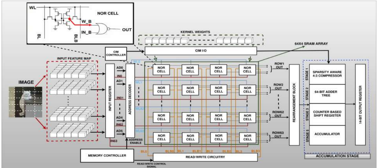
Fig. 1: Proposed 16-Kb SRAM-based digital CIM macro with multi-bank architecture, compute-enabled bit-cells for in-memory MAC operations, and peripheral support including compression, hierarchical adder tree, and control logic for efficient accumulation and output.
