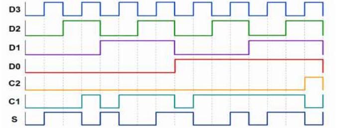
Fig. 5: Functional waveform of the proposed 4-bit full adder.
