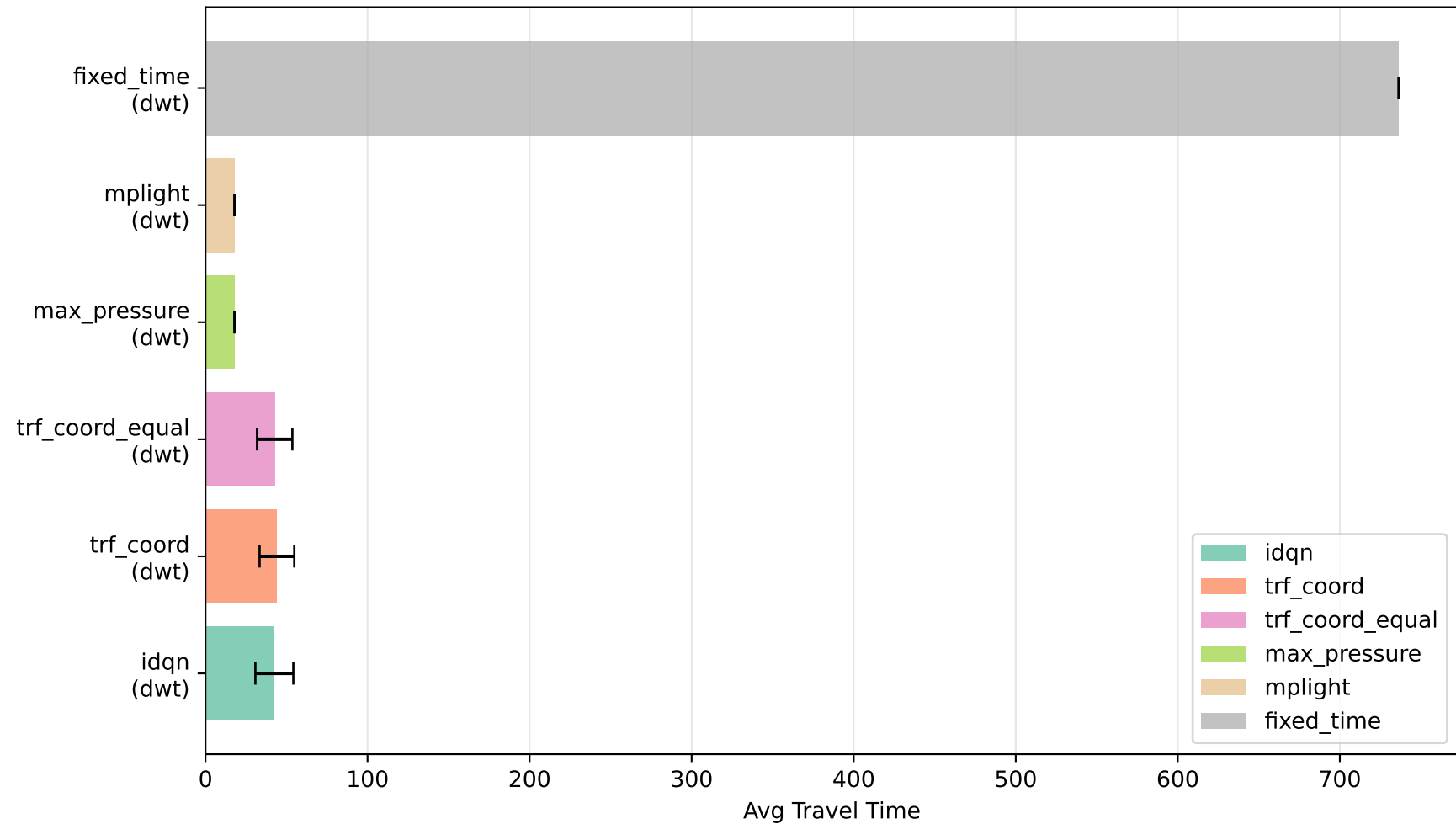
Final Avg Travel Time — grid4x4 / dwt
