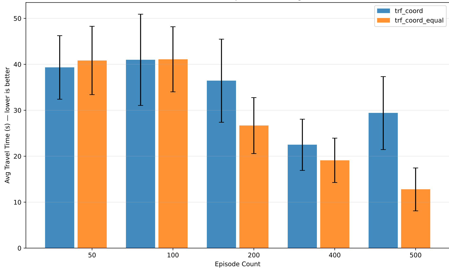
Final Performance vs Episode Count — grid4x4
