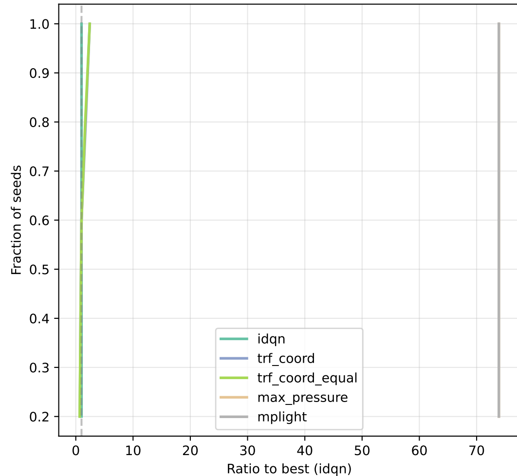
Performance Profile
