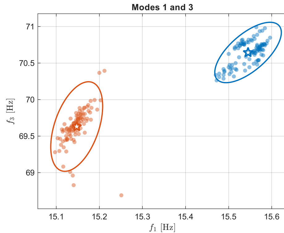
Modal-frequency cross scatter: Porto Alegre (BR) vs Hannover (DE)
