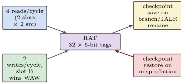
Figure 6: RAT read/write/checkpoint datapath. Writes are gated by a destination-valid flag; slot B's write overrides slot A's on a same-cycle same-register conflict.
