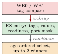
Figure 13: Reservation-station entry lifecycle: wakeup then select. Every entry compares each not-yet-ready operand against both writeback ports independently, every cycle.
