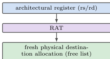
Figure 21: WAR/WAW elimination path. Every destination write allocates a new physical register through this same path, structurally preventing both hazard classes.
