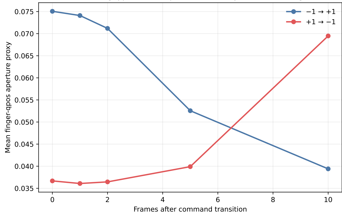
Measured gripper-state response after binary command changes
