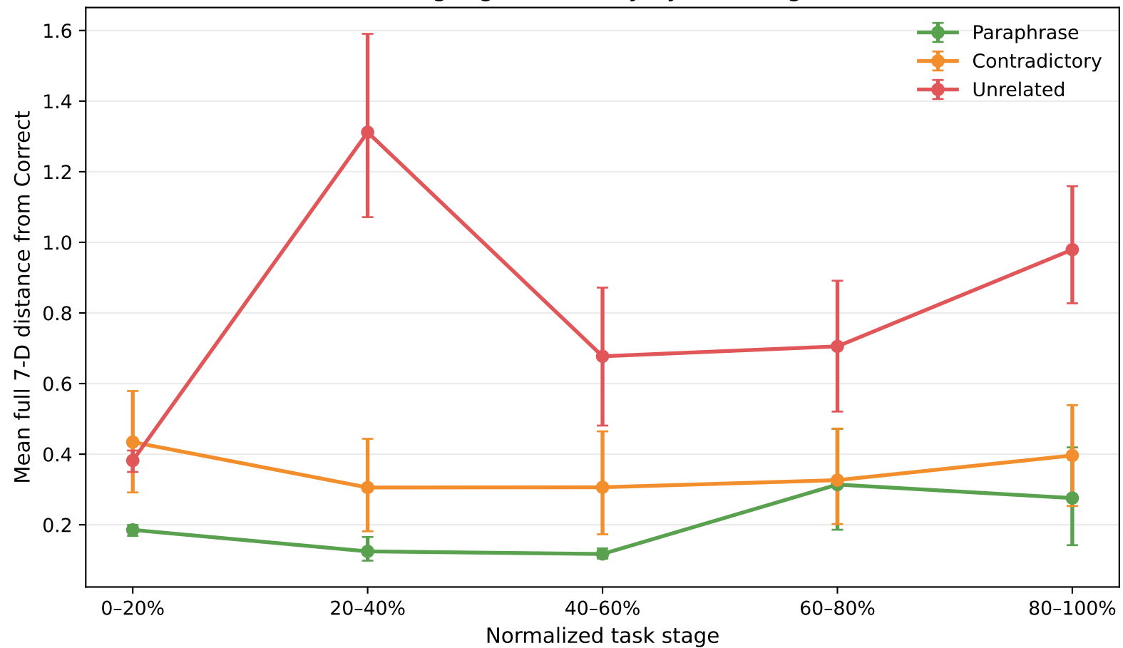
Language sensitivity by task stage
