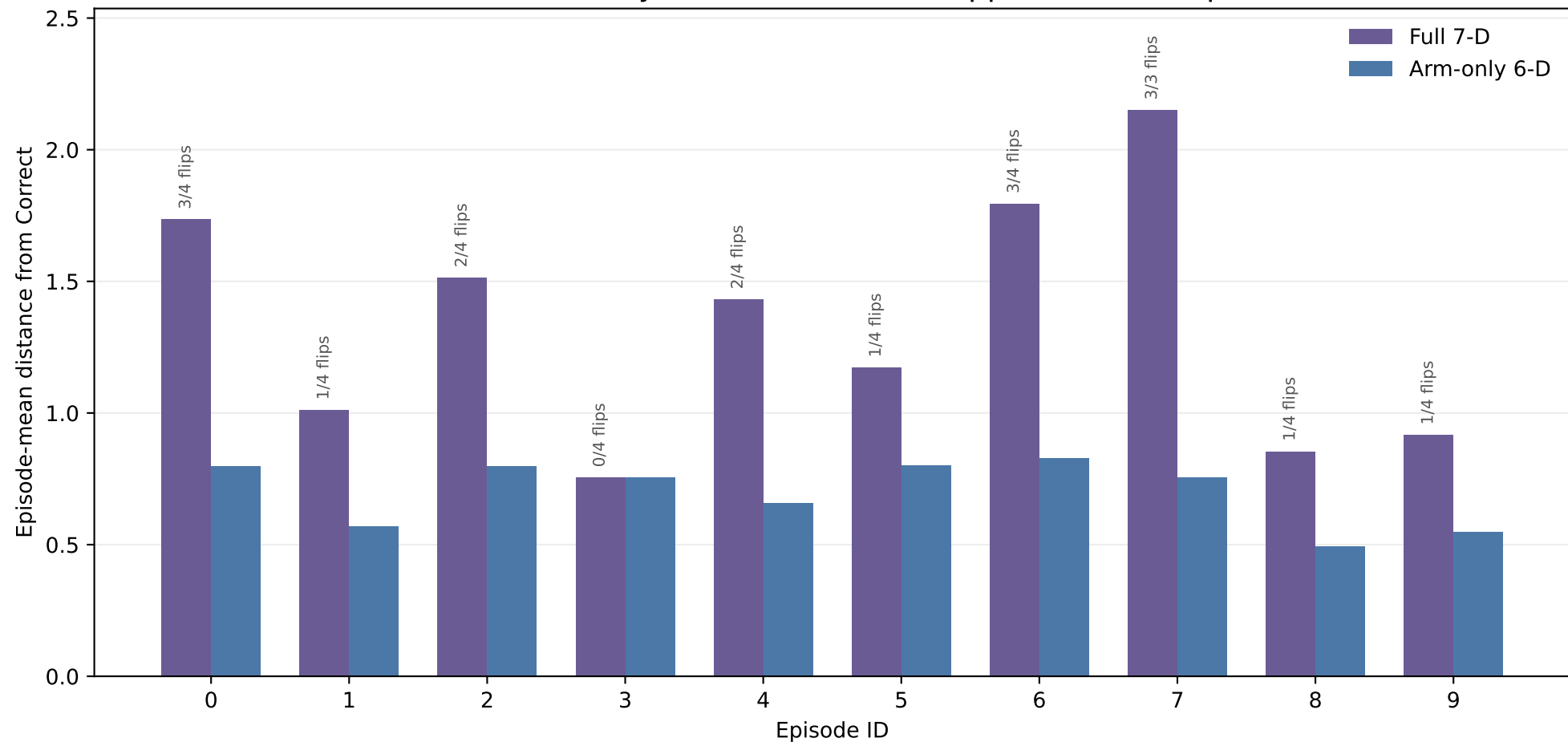
Unrelated Sensitivity in the 20-40% Bin Appears Across Episodes
