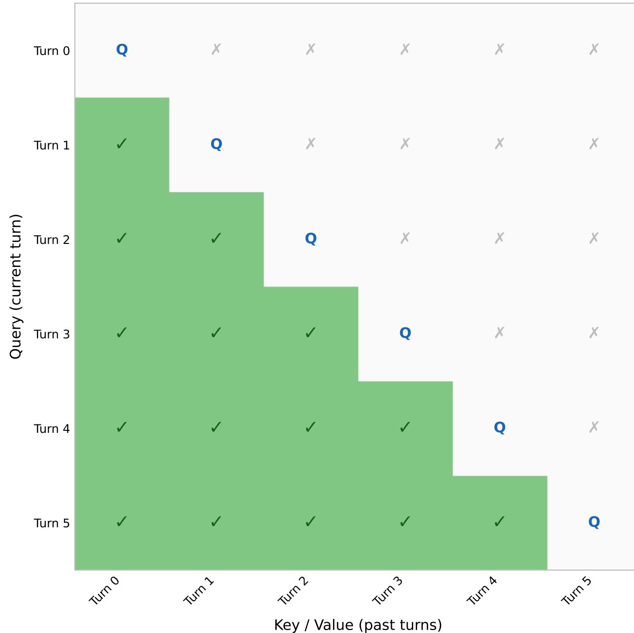
(a) Causal Attention Mask Turn t attends to turns 0..t-1
