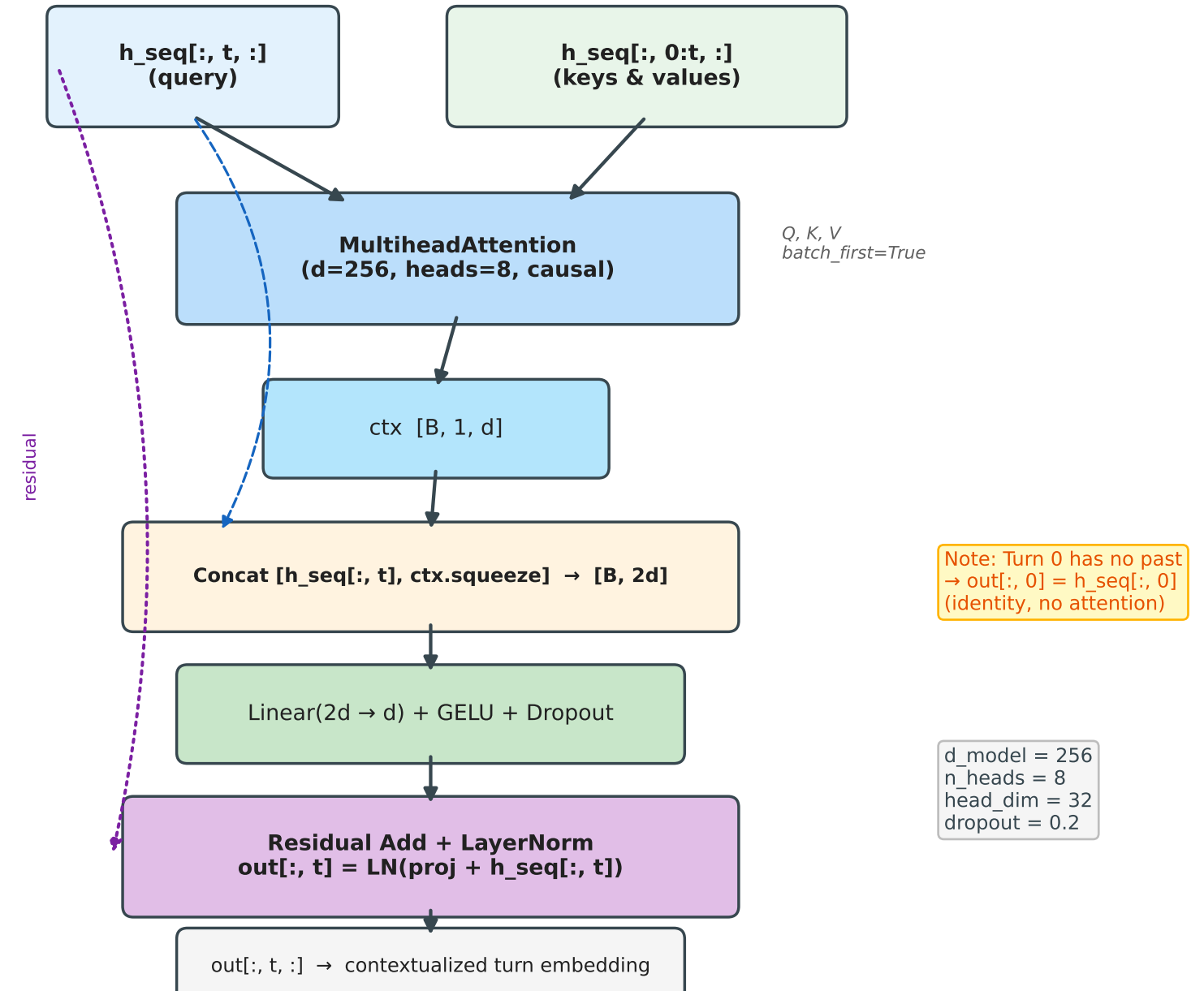
(b) CrossTurnAttention — Processing Turn t
