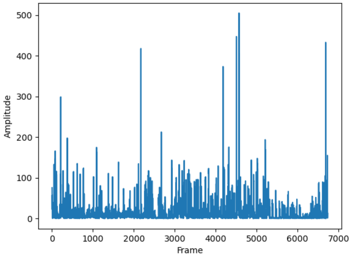
Saccade Amplitudes
