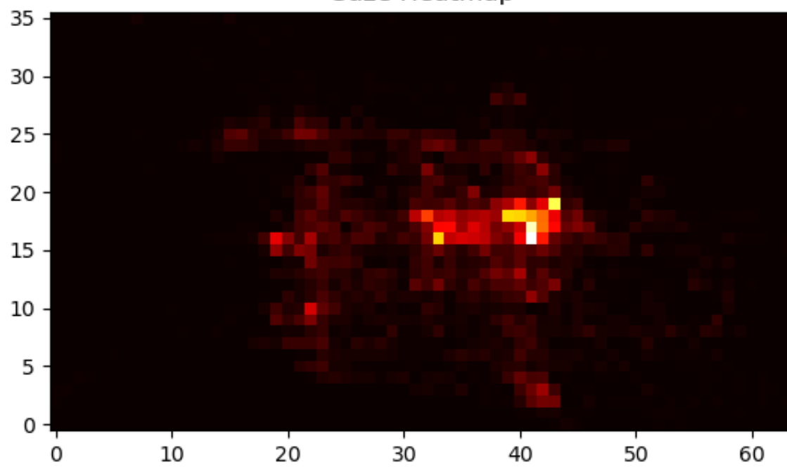
Gaze Heatmap
