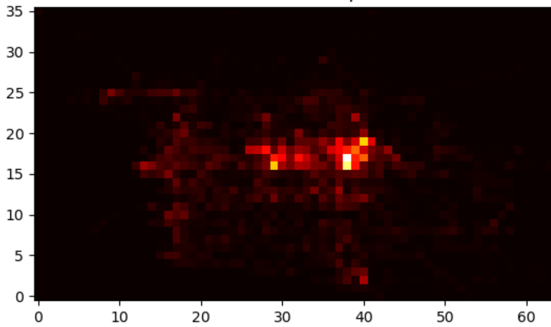
Gaze Heatmap
