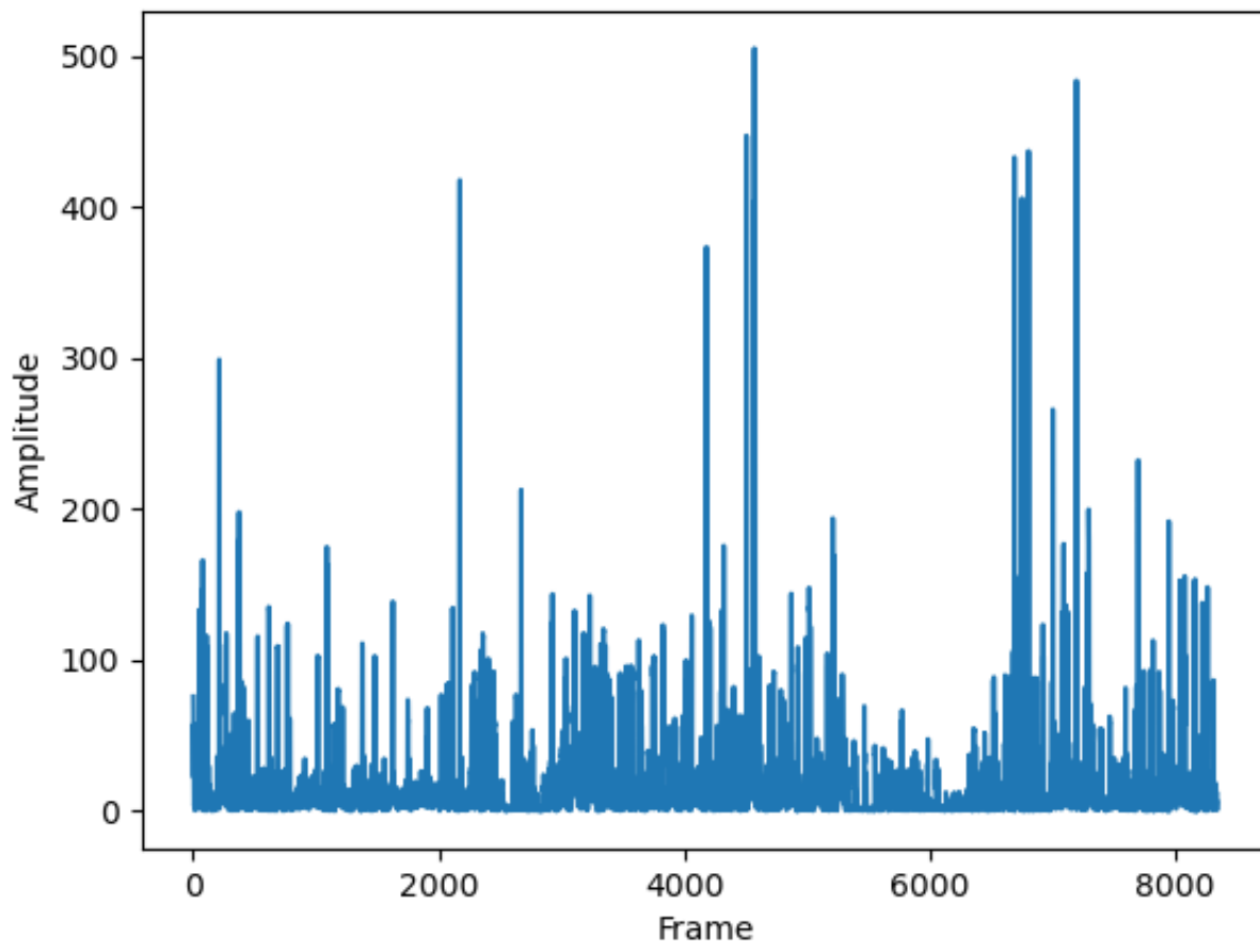
Saccade Amplitudes
