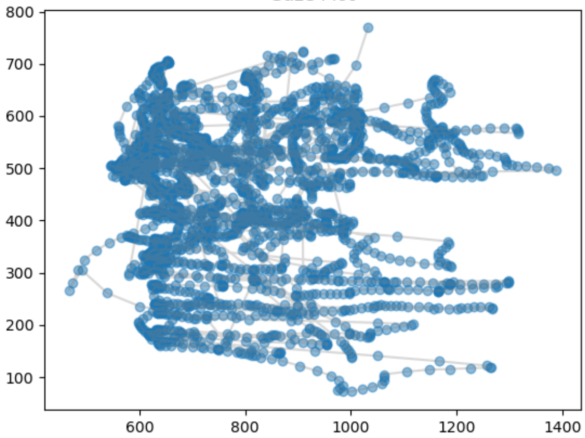
Gaze Plot
