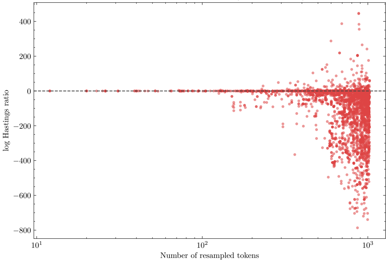
Longer resamples score worse (Spearman -0.45)
