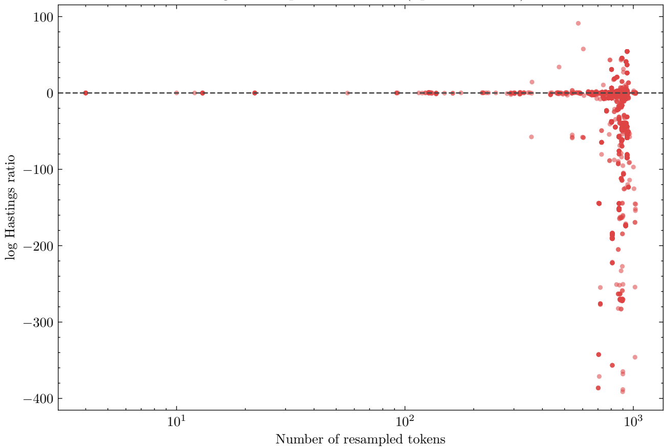
Longer resamples score worse (Spearman -0.10)
