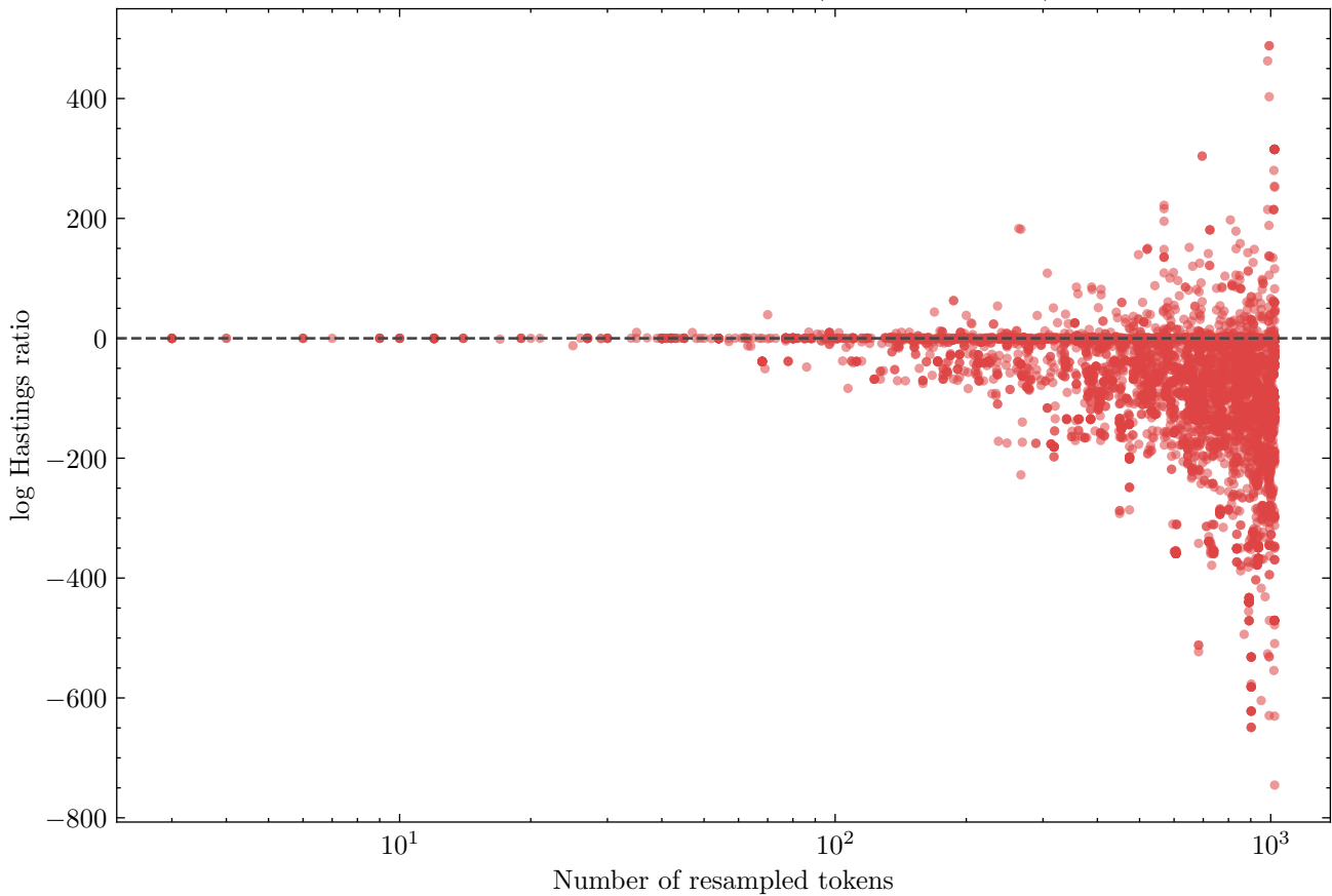
Longer resamples score worse (Spearman -0.33)
