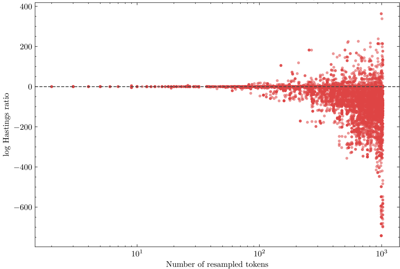
Longer resamples score worse (Spearman -0.43)
