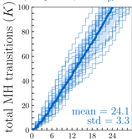
(a) PreSTO-EntropyCut (accept first; best N_{\text{pf}} = 20 )
