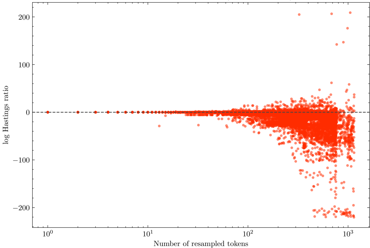
Longer resamples score worse (Spearman -0.52)
