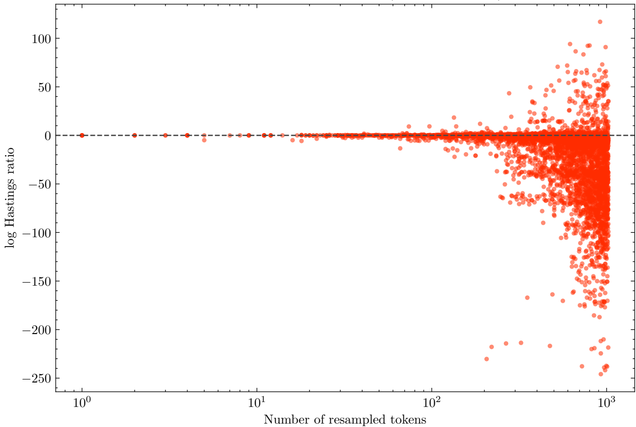
Longer resamples score worse (Spearman -0.49)
