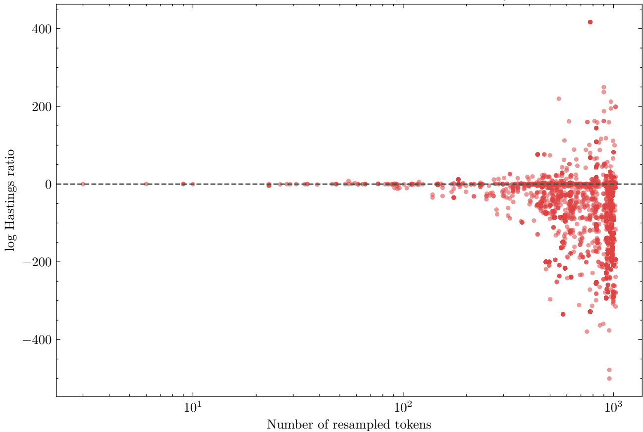
Longer resamples score worse (Spearman -0.34)
