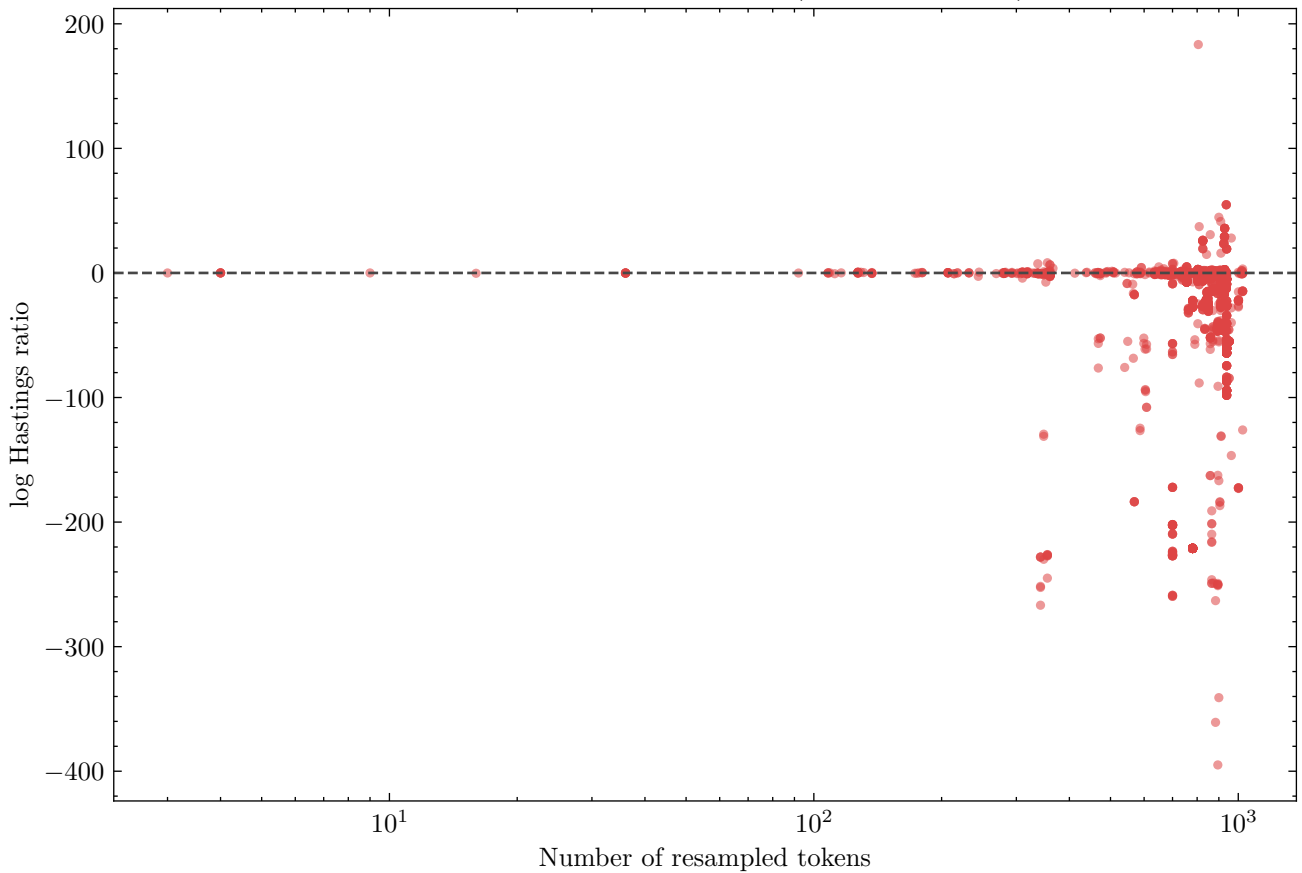
Longer resamples score worse (Spearman -0.14)
