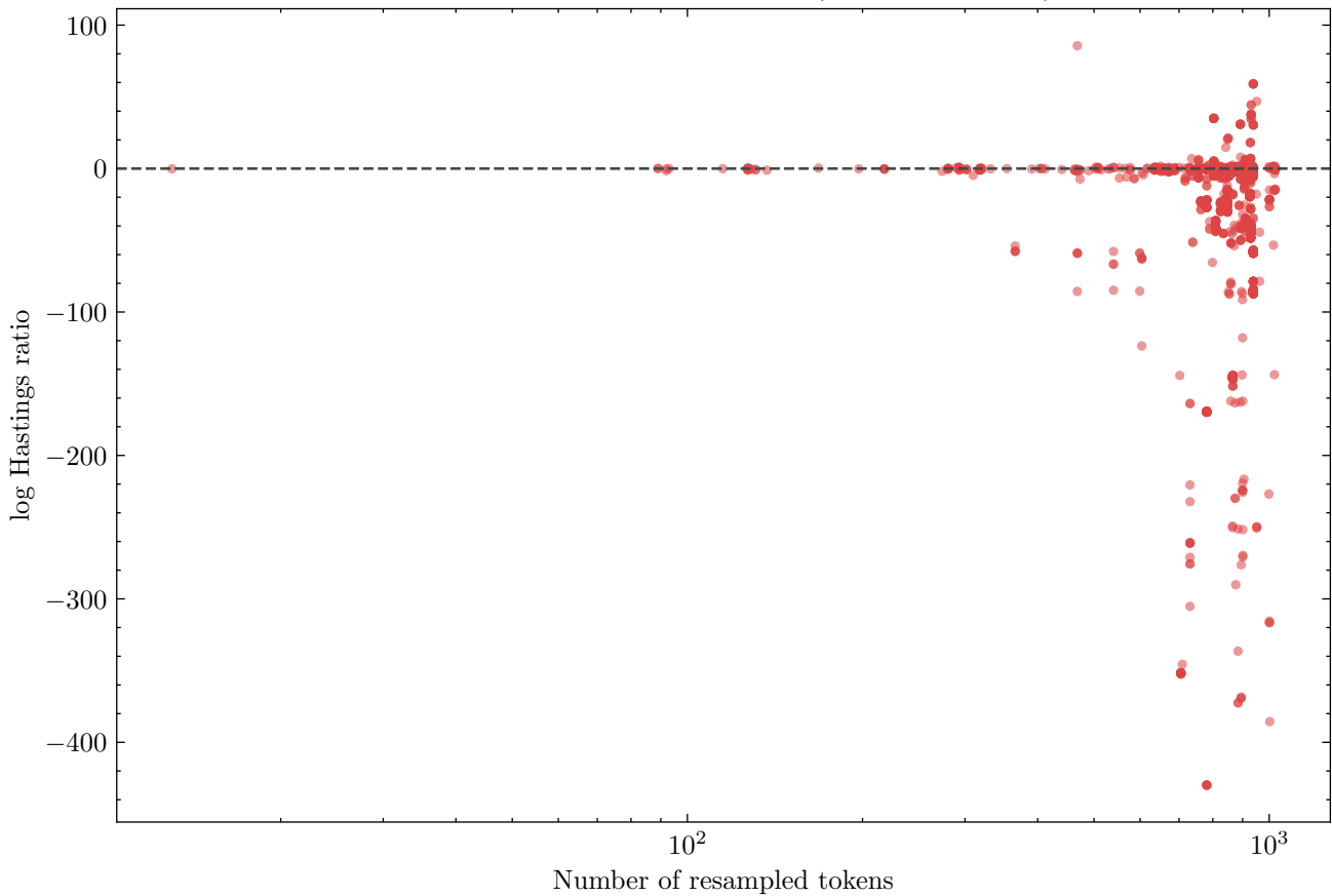
Longer resamples score worse (Spearman -0.01)
