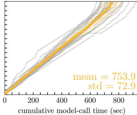
(b) PreSTO-EntropyCut, N_{\text{pf}} = 8 , longest first
