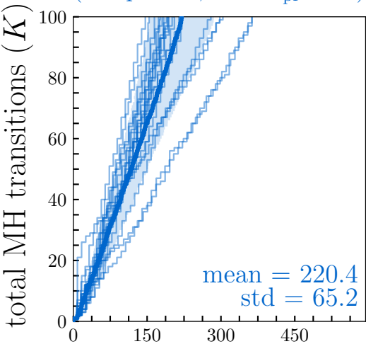
(a) PreSTO-EntropyCut (accept first; best N_{\text{pf}} = 20 )
