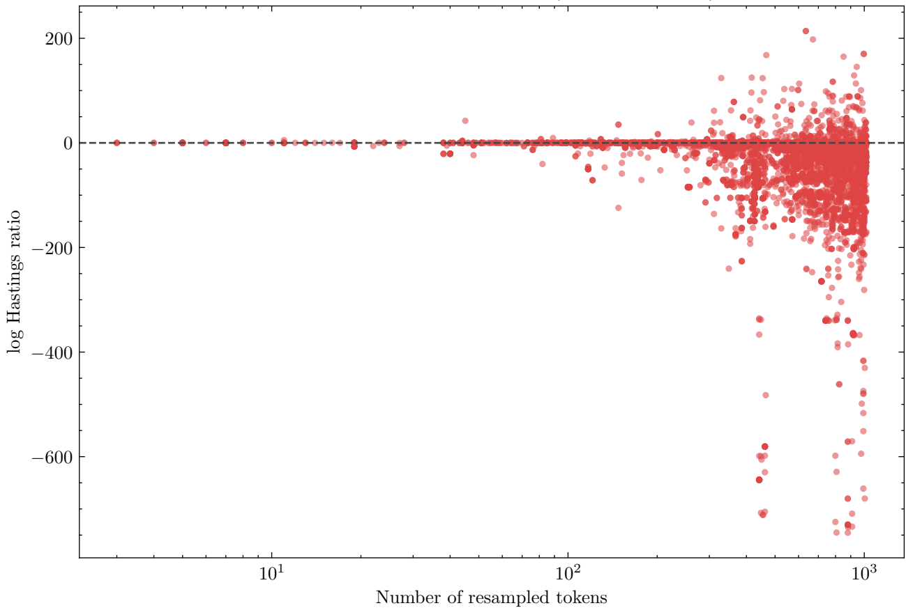
Longer resamples score worse (Spearman -0.40)
