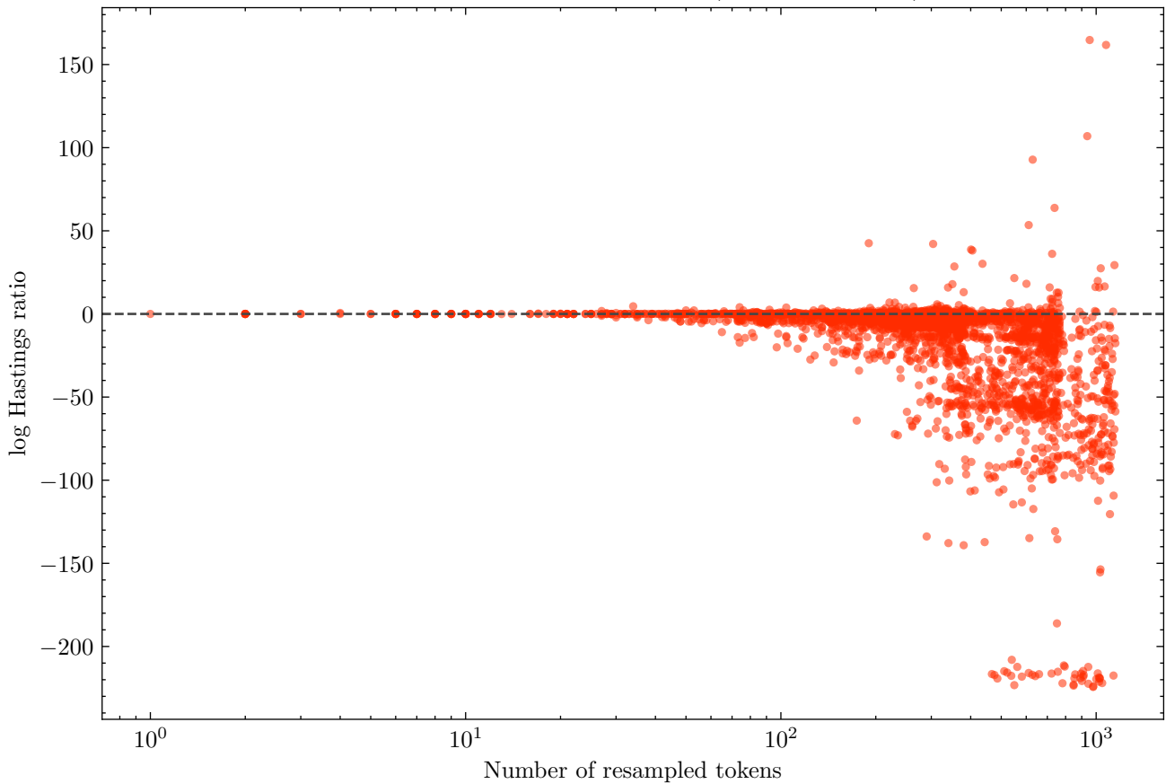
Longer resamples score worse (Spearman -0.58)
