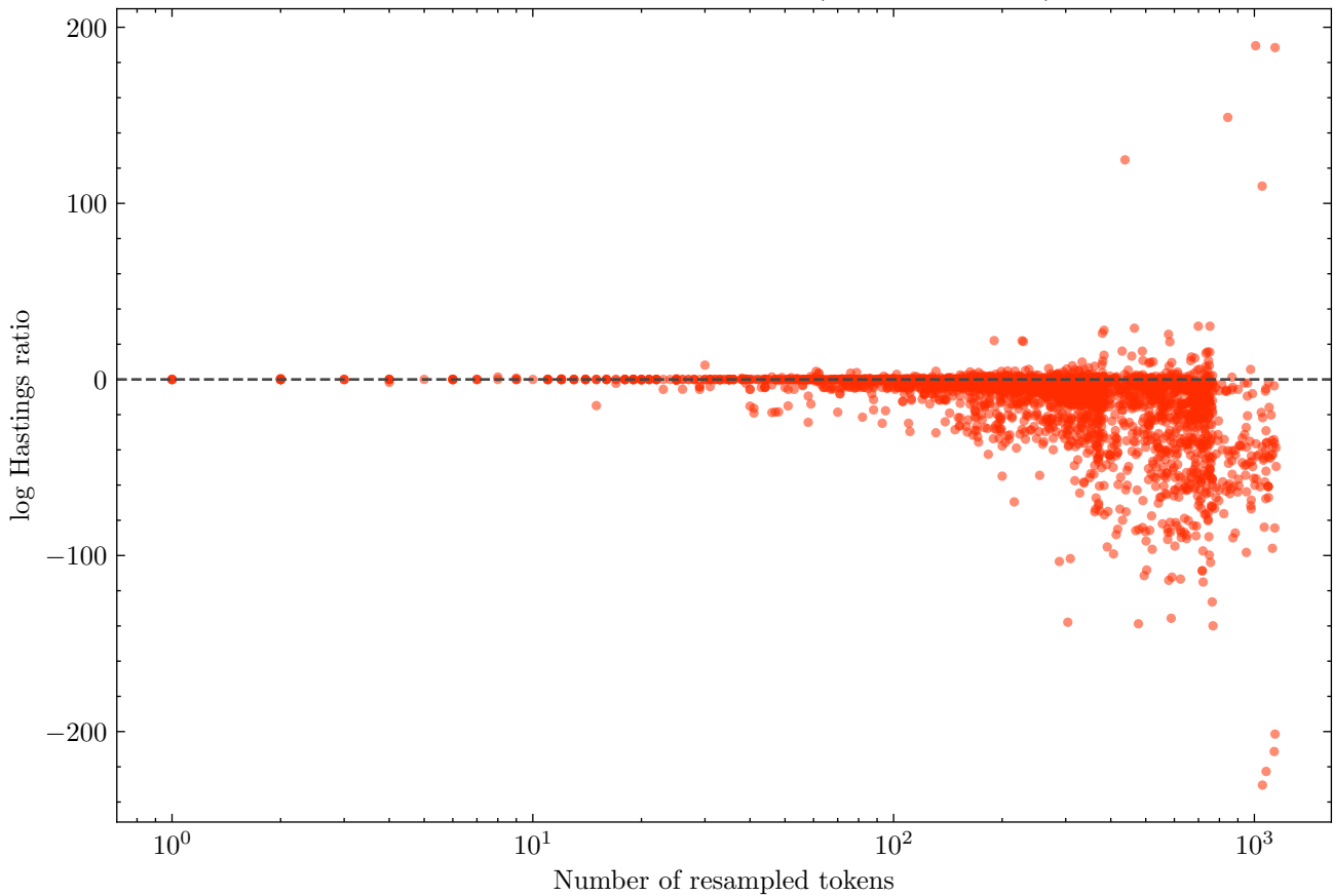
Longer resamples score worse (Spearman -0.50)
