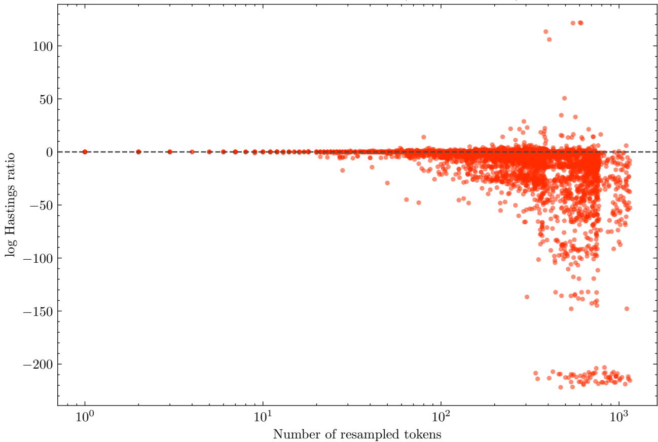
Longer resamples score worse (Spearman -0.53)
