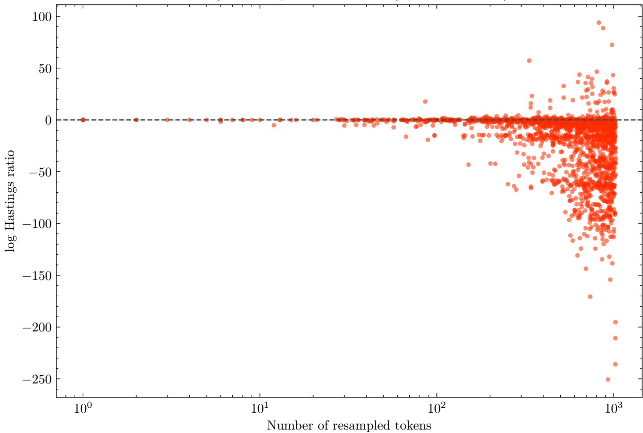
Longer resamples score worse (Spearman -0.46)
