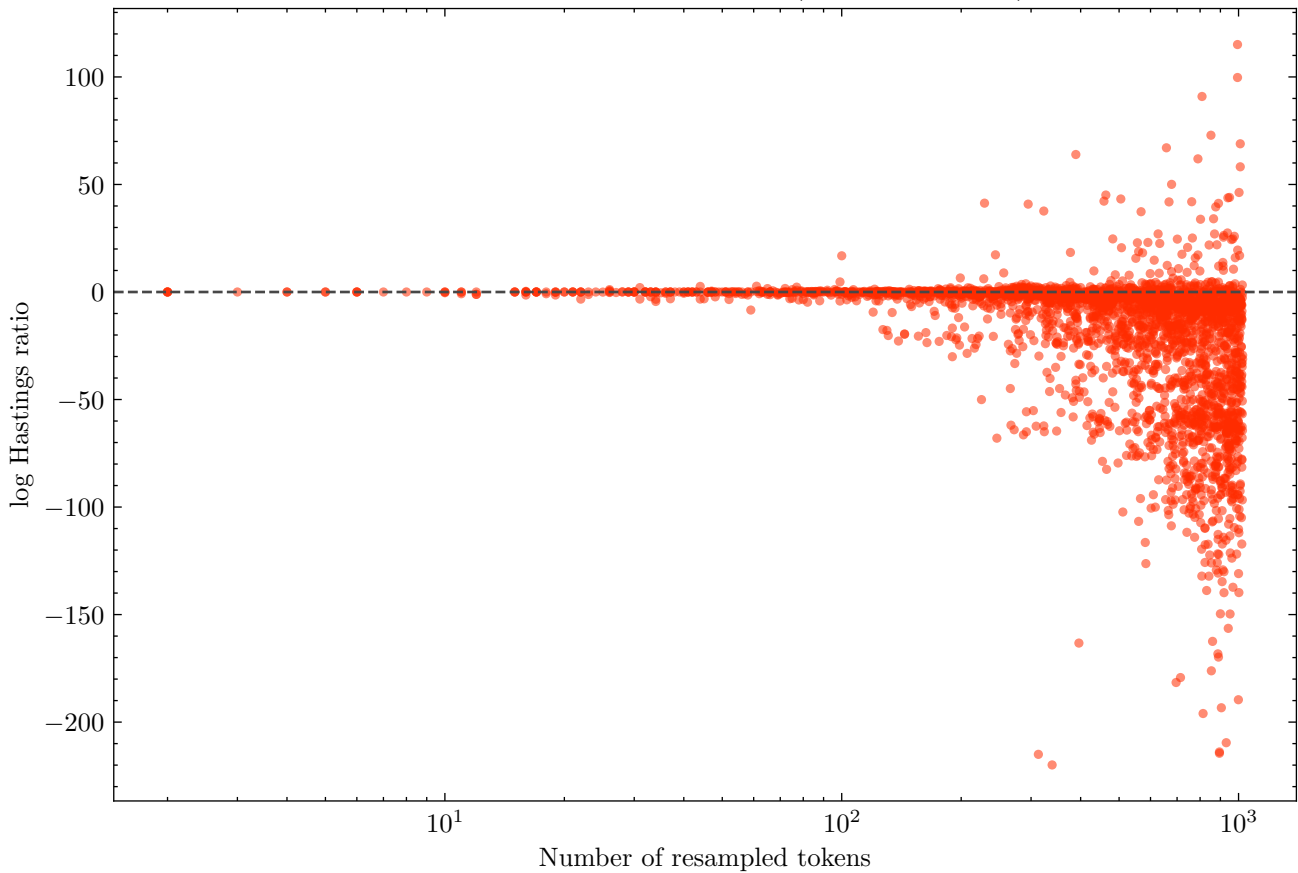
Longer resamples score worse (Spearman -0.56)
