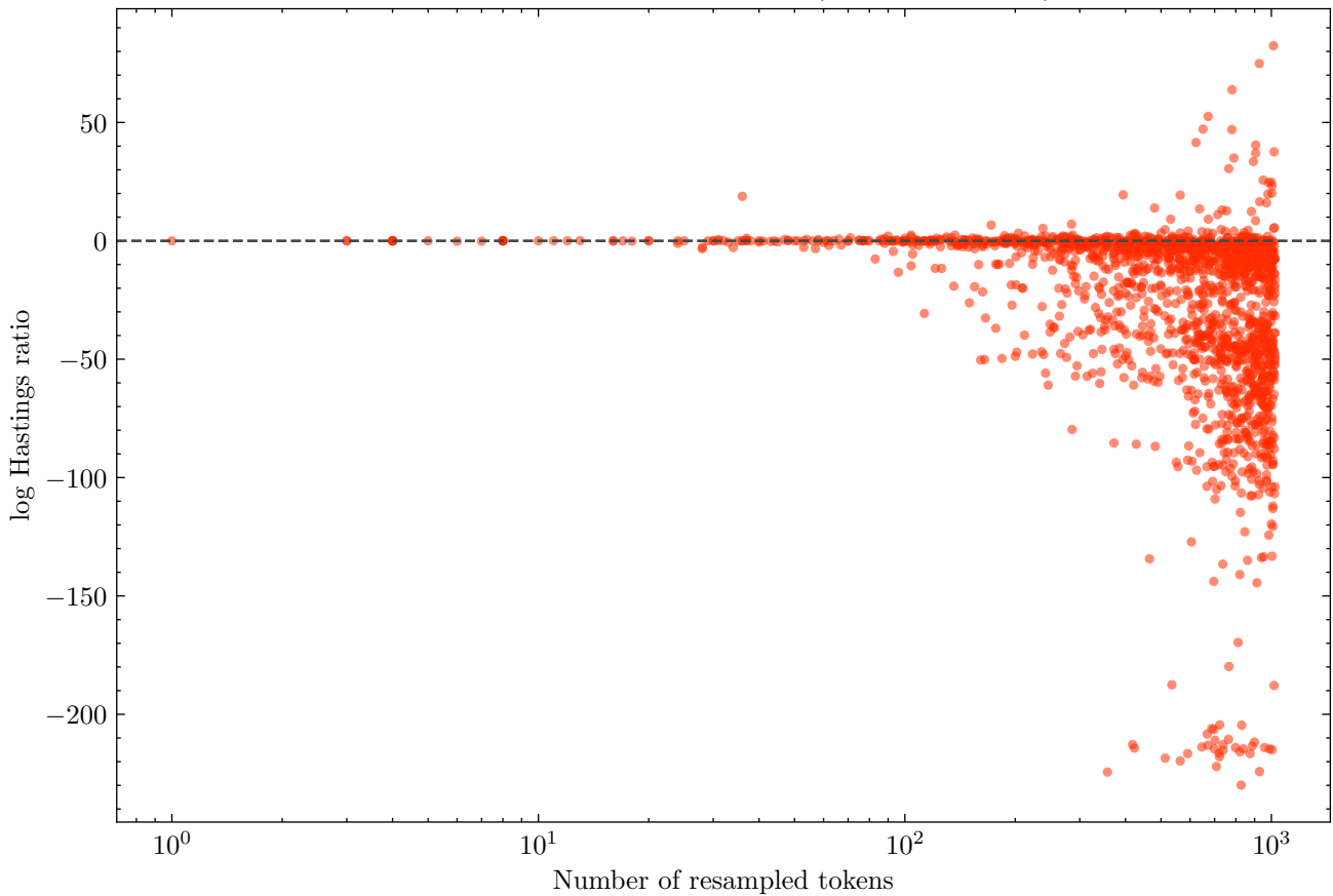
Longer resamples score worse (Spearman -0.48)
