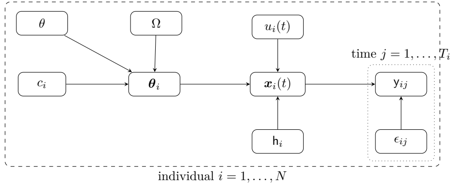
Figure 1: A QSP plate separates the mechanistic state equation from the probabilistic state equation. The mechanistic ODE lives inside \mathbf{x}_i(t) ; the plate tells us how population parameters, individual variation, covariates, latent features, design, and measurement error generate observed biomarkers.
