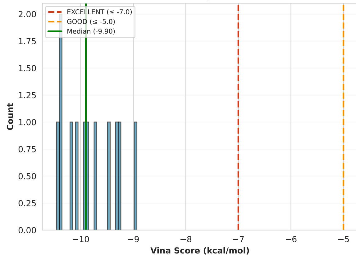
PfCRT 6UKJ (n=12 compounds)
