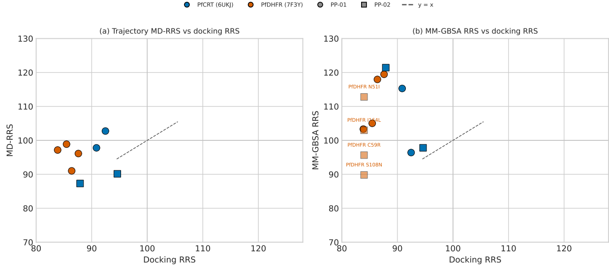
Figure S5: Set-C pilot: trajectory-derived ratios versus docking RRS (wild type = 100). (a) Mean minimum-distance ratios for eight mutants with a docking wild-type reference. (b) MM-GBSA ratios versus docking RRS. Four PP-02 PfdHFR states lack a docking wild-type reference. The dashed diagonal indicates equality; the horizontal and vertical guides indicate the wild-type ratio. Docking predicted weaker mutant scores in the comparable systems; trajectory metrics did not recover that pattern. Neither quantity is a free-energy or experimental resistance measure.
