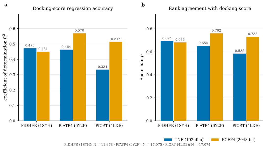
Figure 6: Tartarus docking validation of Tensor Network Embeddings. Random Forest regression performance (100 trees, 5-fold cross-validation) of the 192-dimensional TNE descriptor against the 2048-bit ECFP4 baseline when predicting docking scores for three Plasmodium targets. (a) Coefficient of determination R^2 . (b) Spearman rank correlation between predicted and computed scores. TNE exceeds ECFP4 for PfDHFR ( N = 11\,878 ) and trails it for PfATP4 ( N = 17\,075 ) and PfCRT ( N = 17\,074 ), retaining substantial binding-relevant information at 5.9\times real-atom compression.
