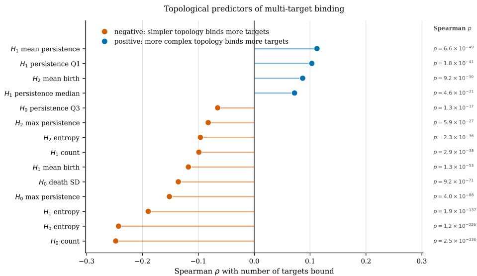
Figure 7: Topological predictors of multi-target binding promiscuity. Spearman correlation between persistent-homology features and the number of Plasmodium targets bound at \Delta G \leq -7.0 \text{ kcal mol}^{-1} , across N = 17\,011 molecules. The 14 interpretable persistence statistics with the largest |\rho| are shown, ordered by \rho , with the corresponding Spearman p -values listed at right. Lower topological complexity accompanies broader target coverage, the strongest negative associations being H_0 count ( \rho = -0.248 ), H_0 entropy ( \rho = -0.243 ) and H_1 entropy ( \rho = -0.190 ), all p < 10^{-137} . A further 45 vectorised persistence-image and Betti-curve components were also tested ( \rho between -0.111 and +0.139); they are omitted here because their individual indices are not chemically interpretable. The underlying analysis reports no confidence intervals, so none are drawn.
