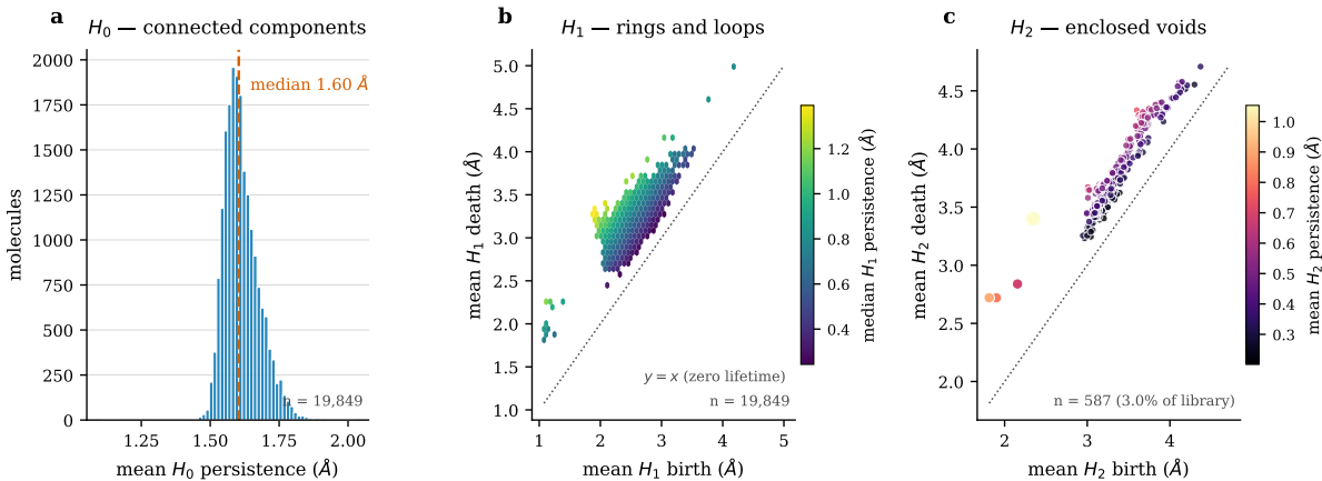
Figure 1: Population-scale persistent homology for the 19 849-molecule ANP-space library (Vietoris–Rips filtration on the weighted interatomic distance matrix). (a) H_0 , connected components: distribution of per-molecule mean H_0 persistence; birth is identically zero for H_0 by construction, and the dashed line marks the median (1.60 \text{\AA} ). (b) H_1 , rings and loops: hexbin density of per-molecule mean (birth, death) coordinates on linear axes, coloured by median H_1 persistence. (c) H_2 , cavities and voids: the 587 molecules (3.0 % of the library) carrying at least one H_2 feature, sized by H_2 count and coloured by mean H_2 persistence. In panels (b) and (c) the dotted diagonal y = x marks zero lifetime; vertical distance from it encodes persistence.
