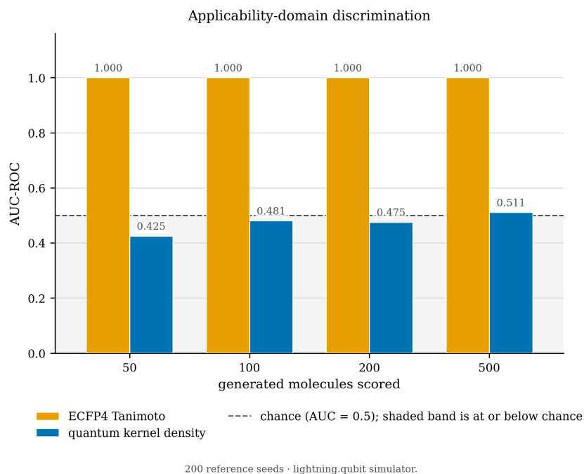
Figure 4: Chemical similarity vs. quantum kernel density discriminator benchmark. AUC-ROC for separating N STONED-SELFIES-generated molecules from 200 reference seeds, scoring each molecule either by its maximum ECFP 4 Tanimoto similarity to a seed (orange) or by its mean quantum kernel density over the reference set (blue). The dashed line marks chance performance ( AUC = 0.5 ) and the shaded band covers performance at or below chance ( AUC = 0.425 – 0.511 ). Simulated on lightning.qubit .
