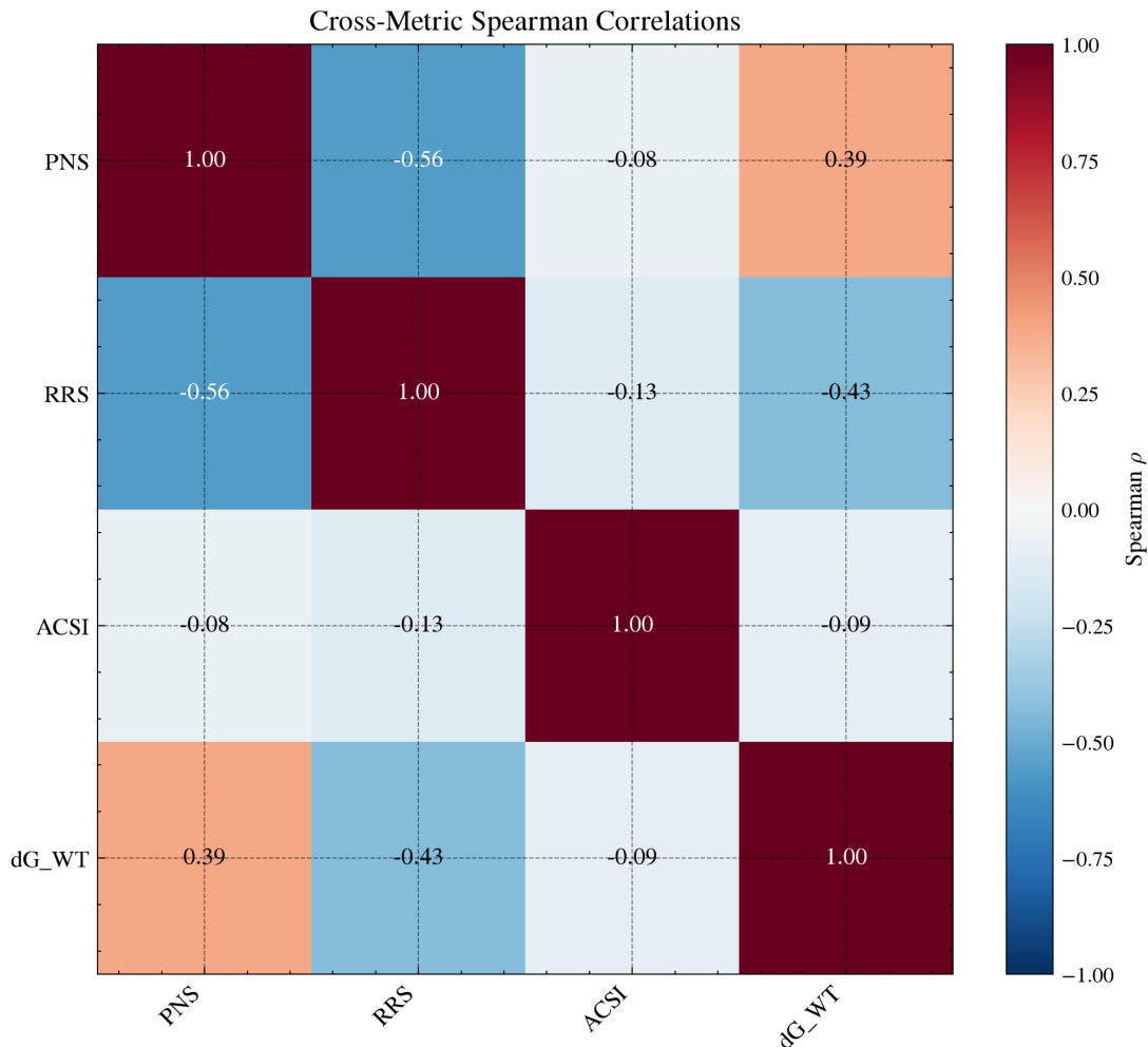
Figure 5: Cross-metric correlation matrix for the 17 polypharmacological candidates with complete data. Spearman \rho values between PNS, ACSI, RRS, and \Delta G_{\text{WT}} . PNS vs. \Delta G_{\text{WT}} shows \rho = +0.389 due to mechanical linkage (see text). None of the hypotheses survive Bonferroni correction ( \alpha = 0.05/3 \approx 0.017 ).
