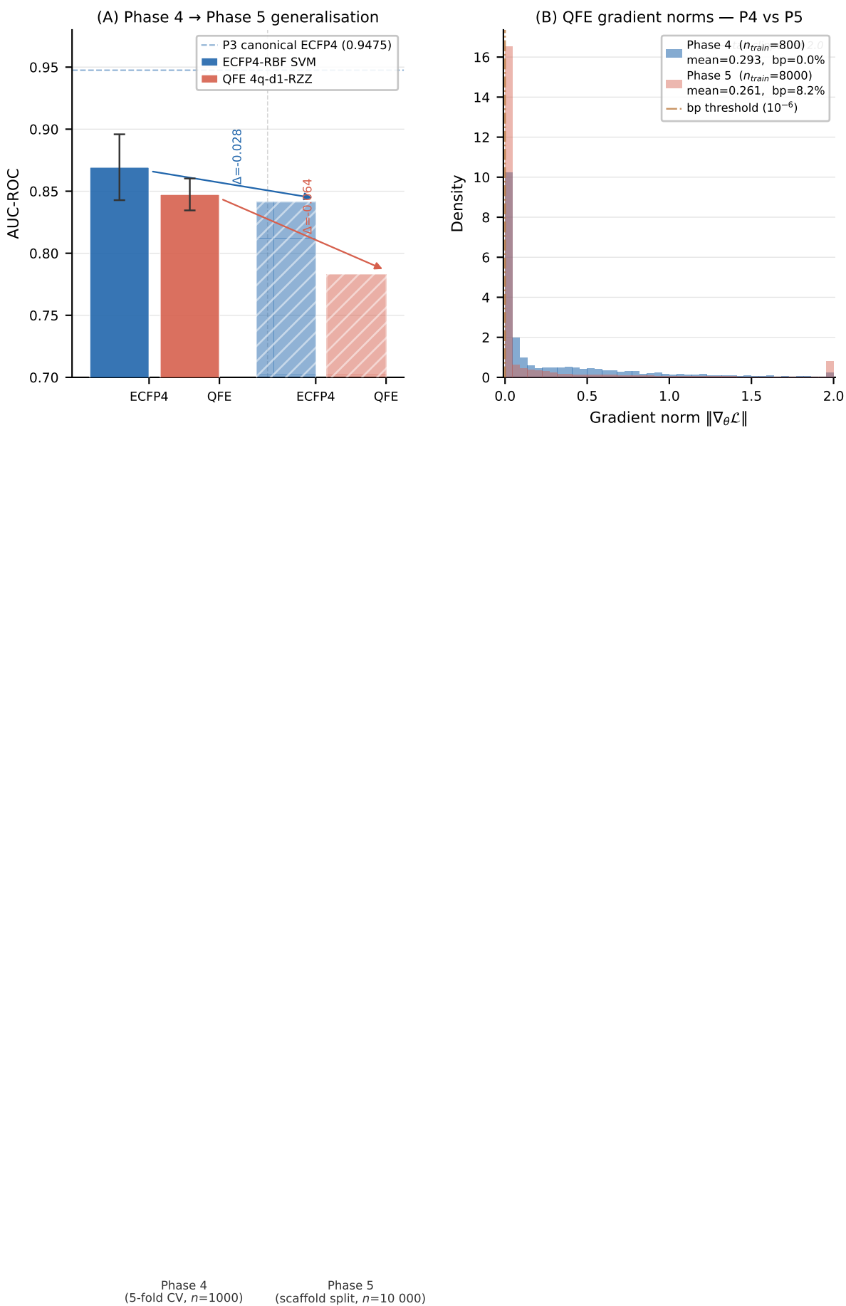
Figure 5. Phase 5 scaffold-split generalisation and gradient diagnostics
